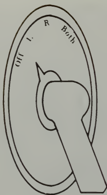
FIGURE 4-14. Switch positions for one ignition switch that controls two magnetos.
